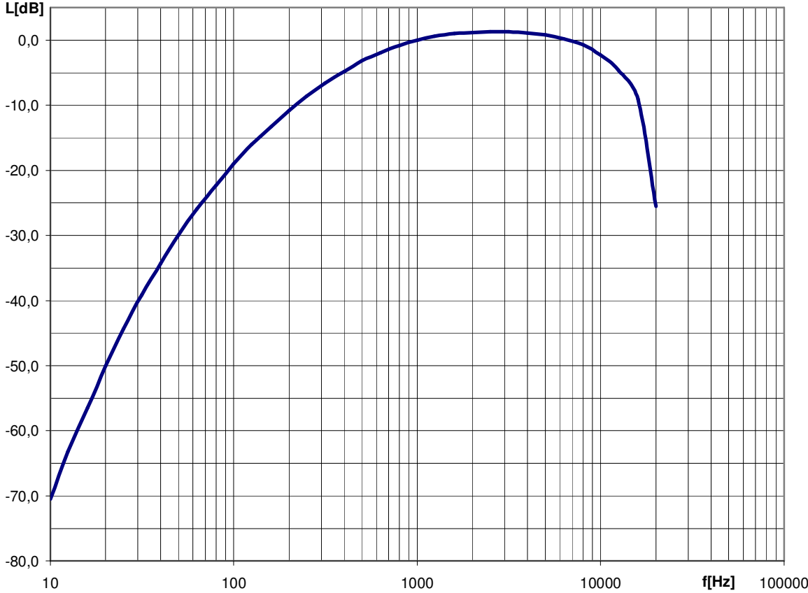
Fig. A.1. The characteristics of A filter, conformable to EN 61672-1:2003 class 1 requirements.
