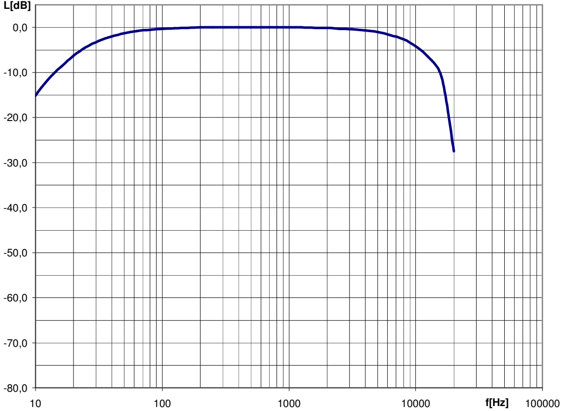
Fig. A.2. The characteristics of C filter, conformable to EN 61672-1:2003 class 1 requirements.
