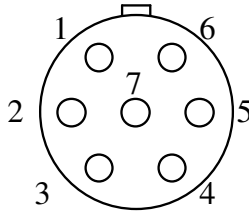
Fig. 2.1. Microphone connector external view.
