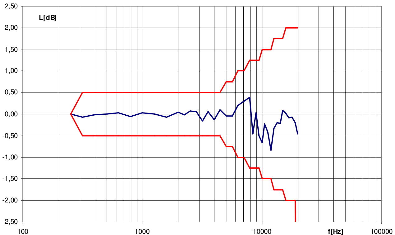
Fig. 1.4. Typical free-field frequency response of WK-21 microphone.
